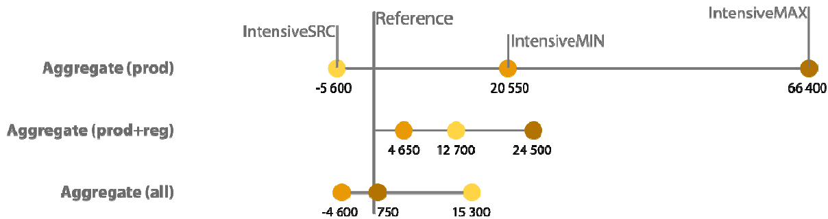
Fig. 3: Comparison of aggregation based on (1) only provisioning services, (2) provisioning and regulating services, and (3) all selected ecosystem services.
